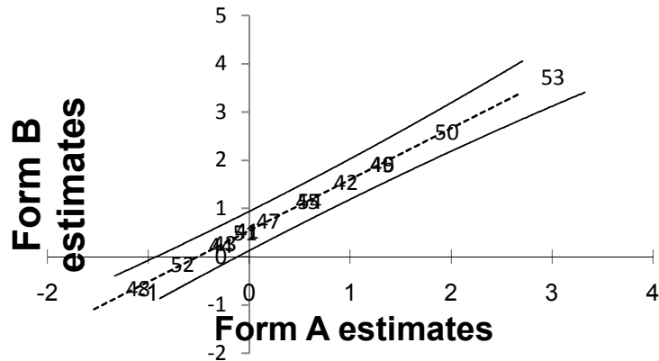
Figure 3 – Cross plot of common items' difficulty estimates based on the two forms
